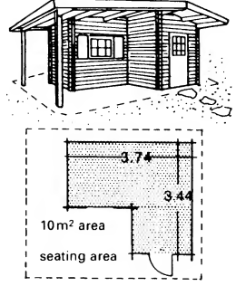
④ Log cabin
